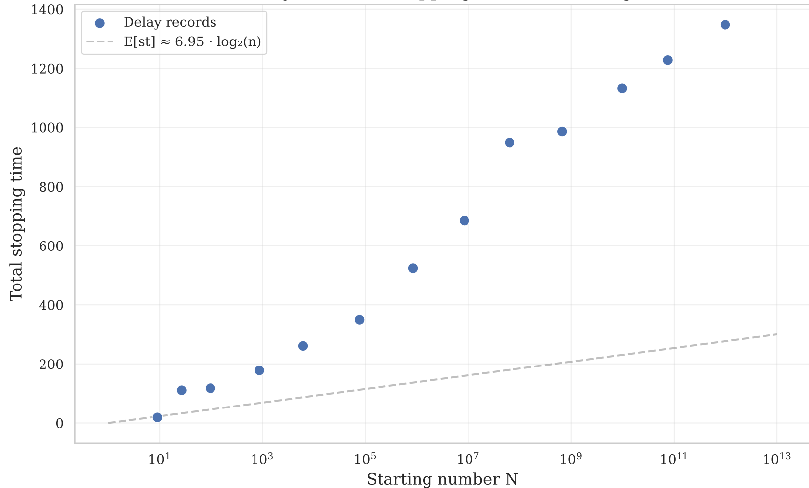
Collatz Delay Records: Stopping Time vs Starting Number
