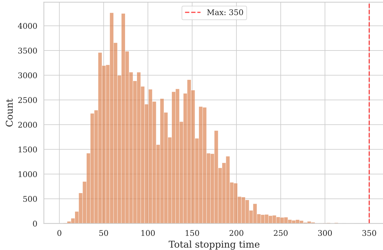
Stopping Time Distribution (n ≤ 100,000)
