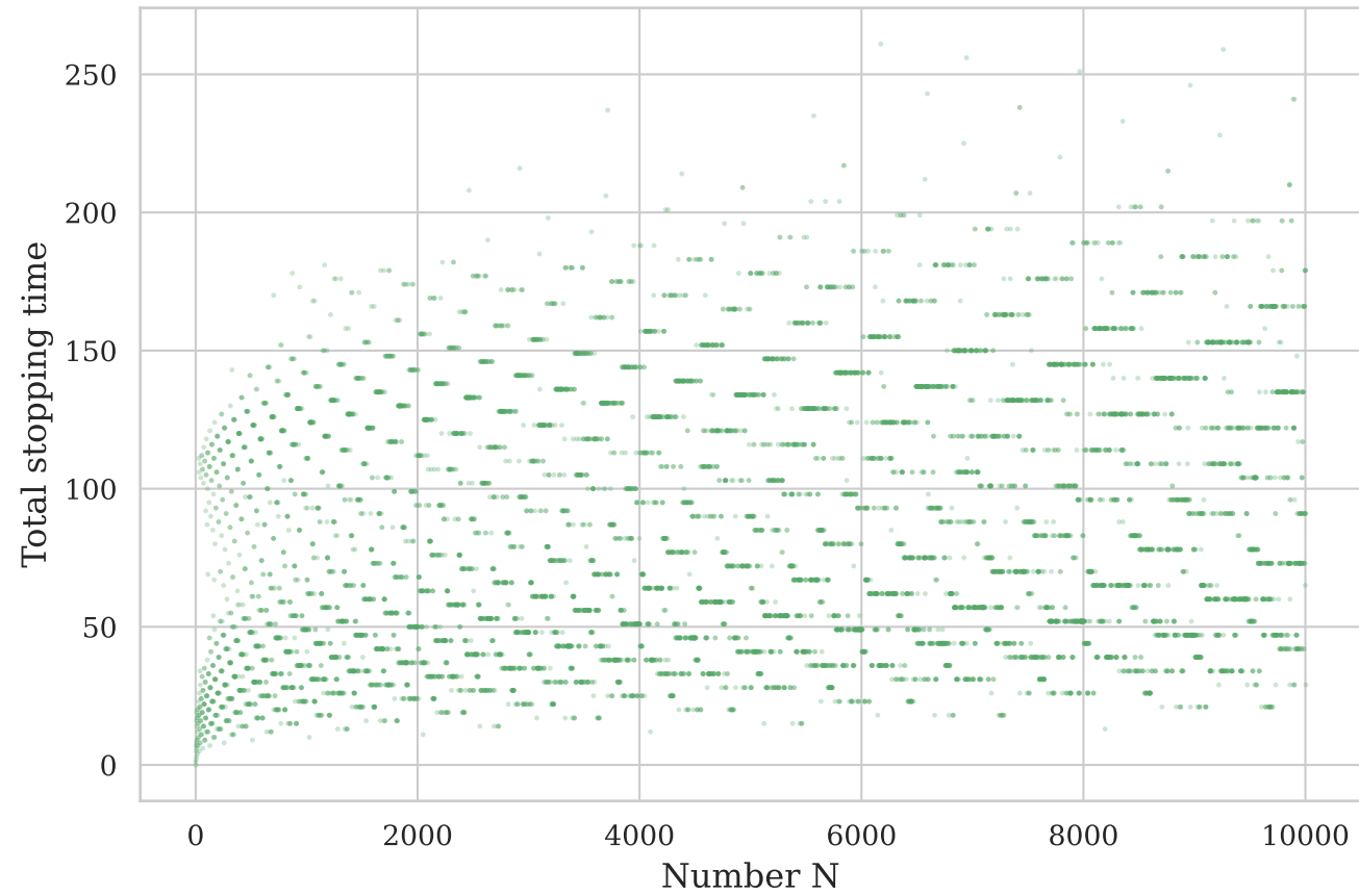
Stopping Times (n ≤ 10,000)
