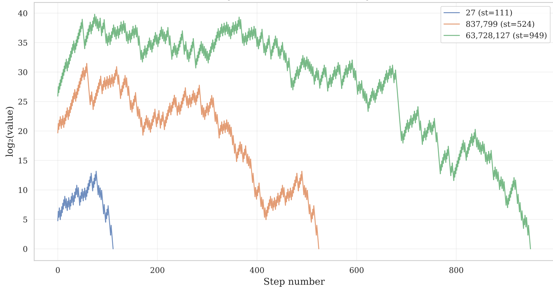
Collatz Trajectories of Notable Delay Records
