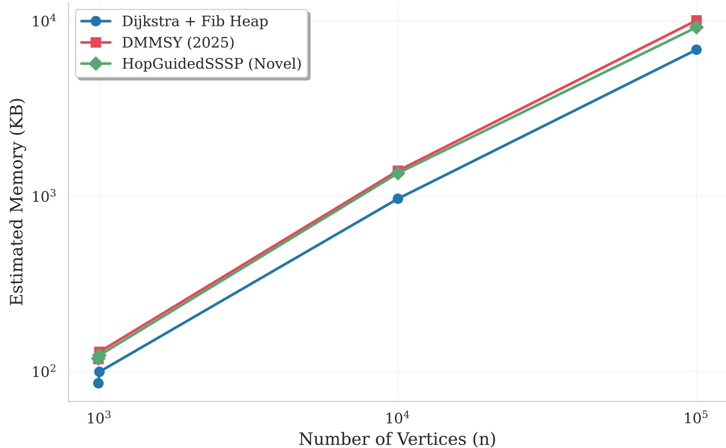
Memory Usage Comparison (Estimated)
