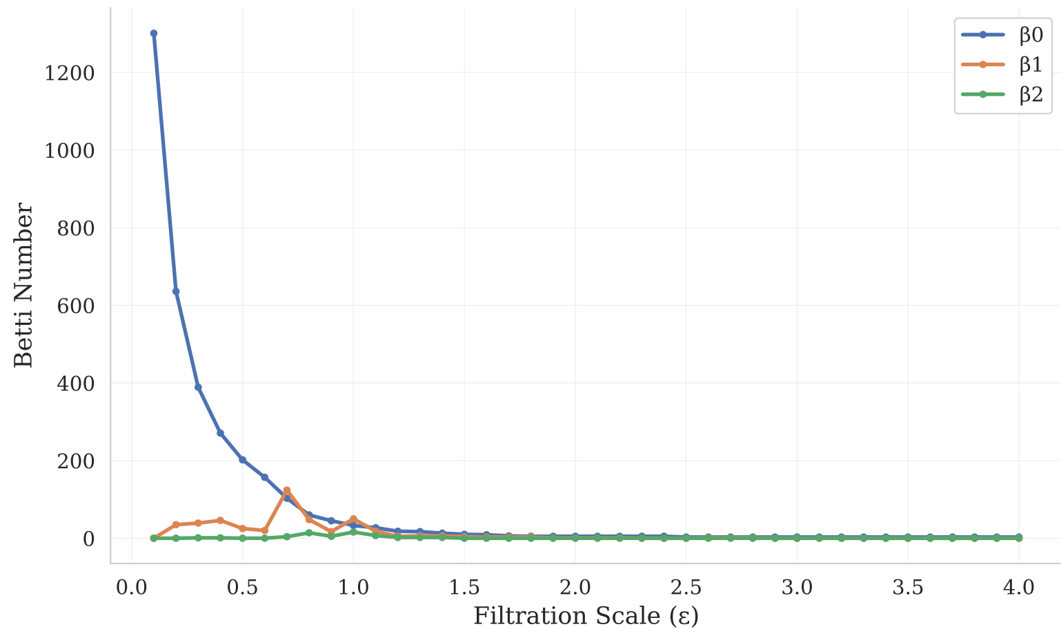
Betti Numbers vs. Filtration Scale
