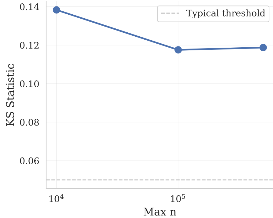
Lyapunov Non-Gaussianity
