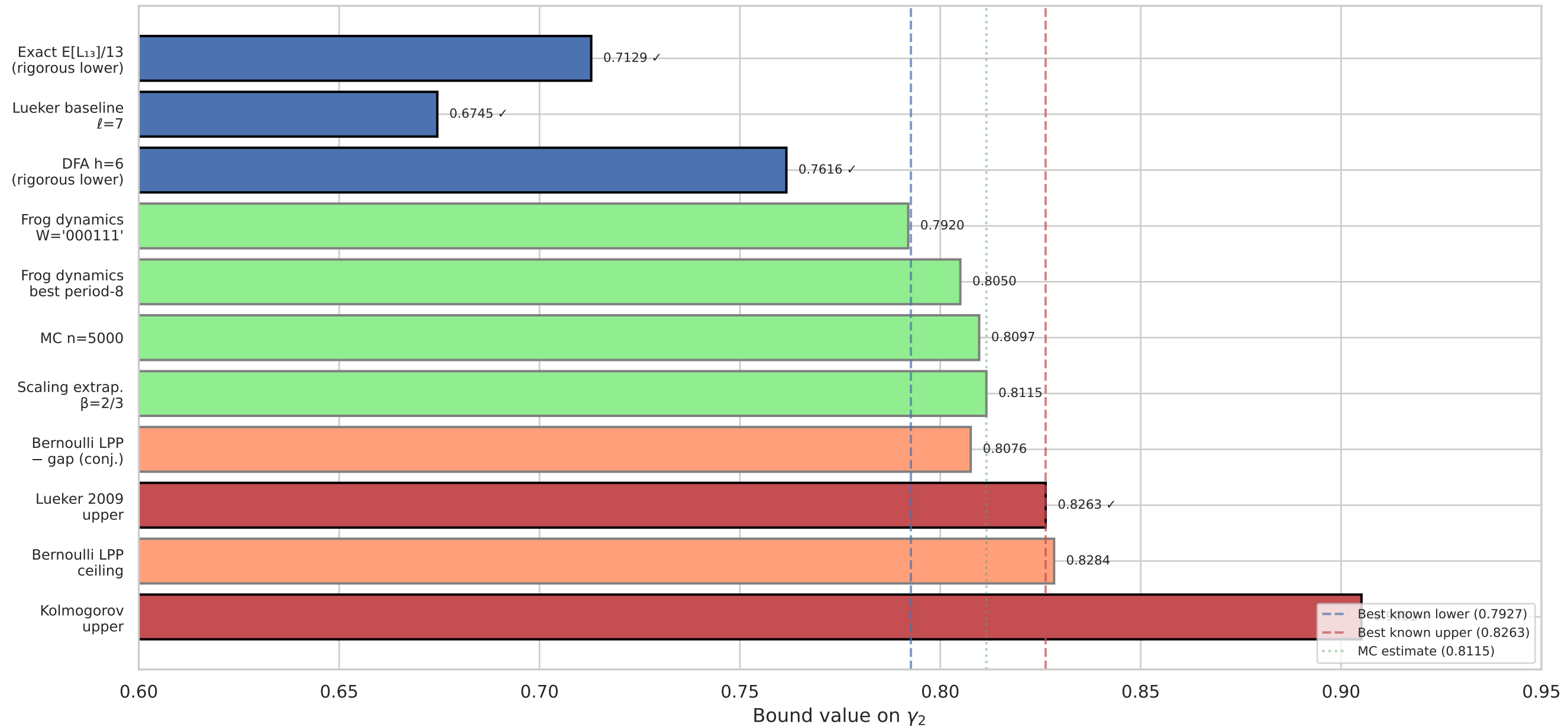
Comparison of All Computed Bounds on \gamma_2
