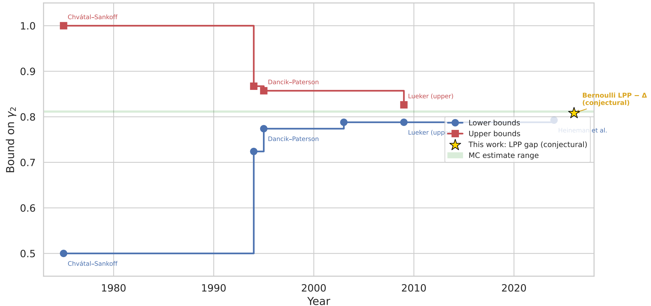
Historical Progression of Bounds on the Binary Chvátal-Sankoff Constant \gamma_2
