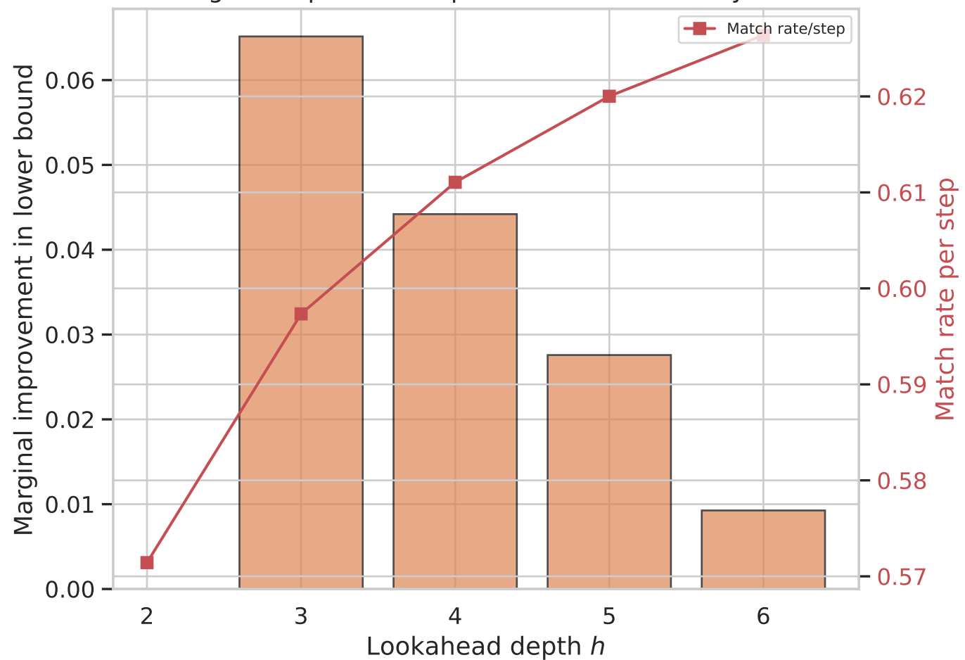
Marginal Improvement per Extra Lookahead Symbol
