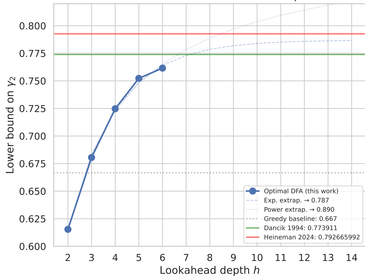
DFA Lower Bound vs. Lookahead Depth
