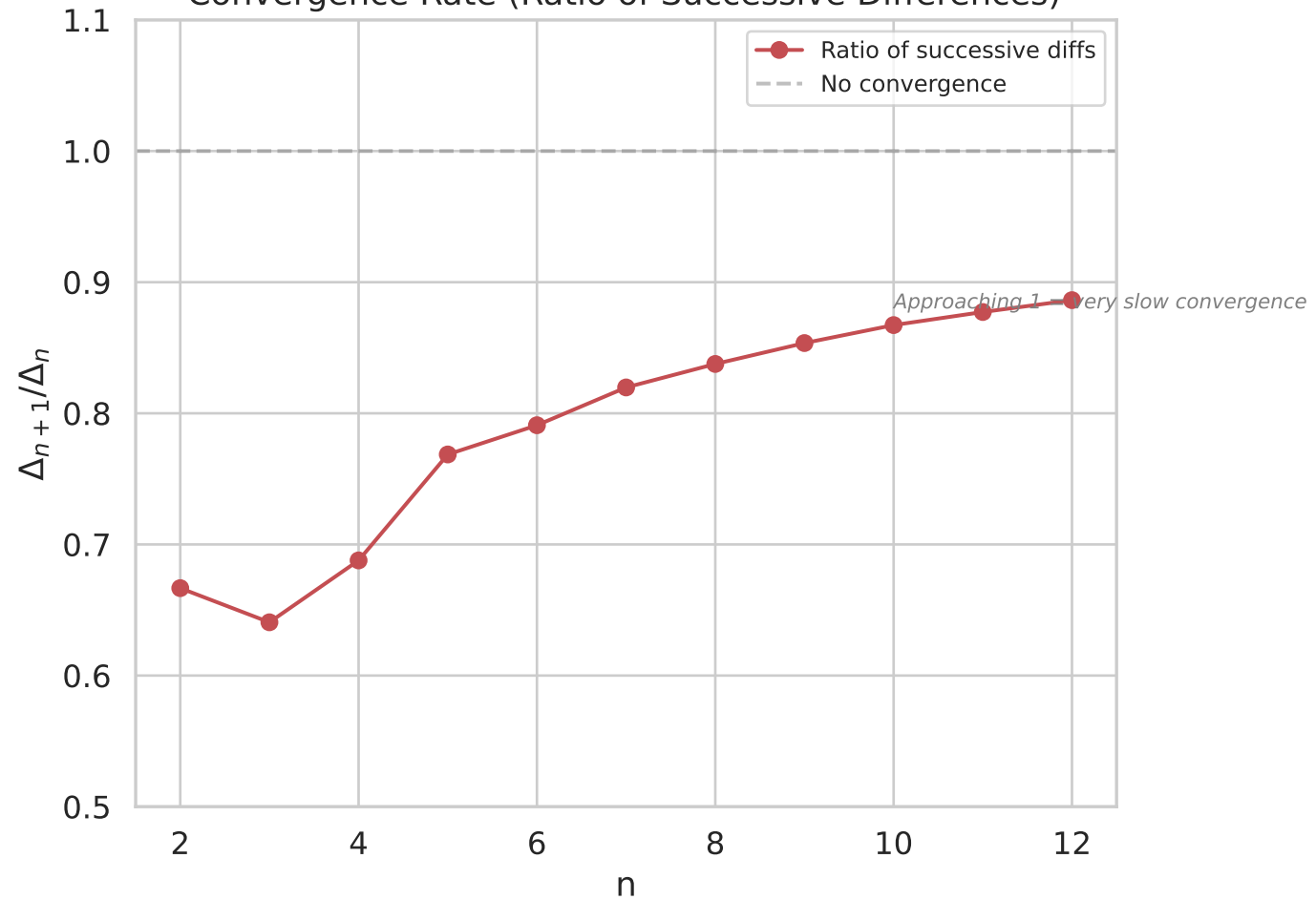
Convergence Rate (Ratio of Successive Differences)
