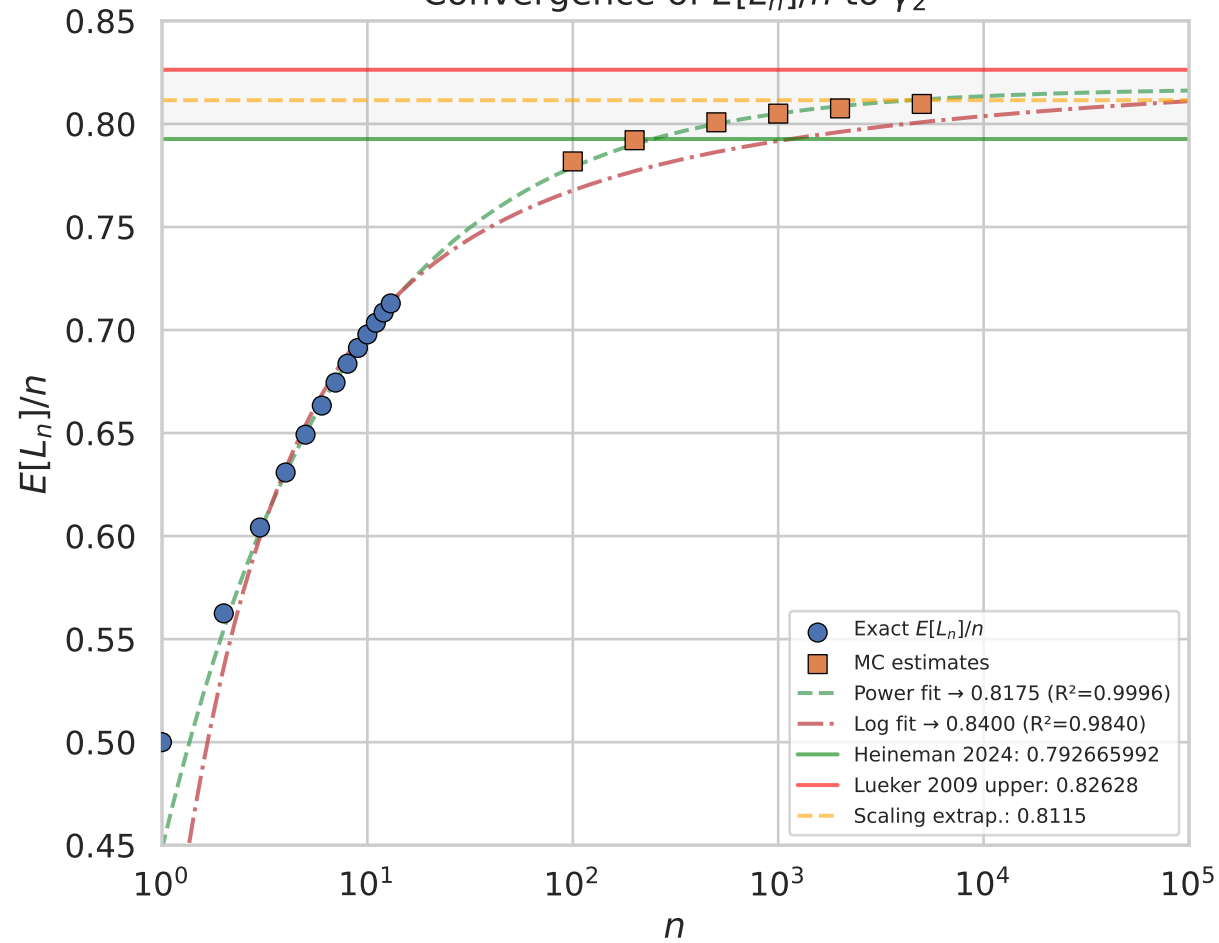
Convergence of E[L_n]/n to \gamma_2
