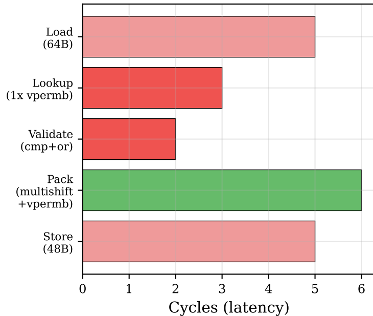
AVX-512 VBMI Decode Pipeline
