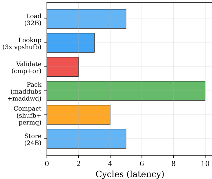
AVX2 Decode Pipeline
