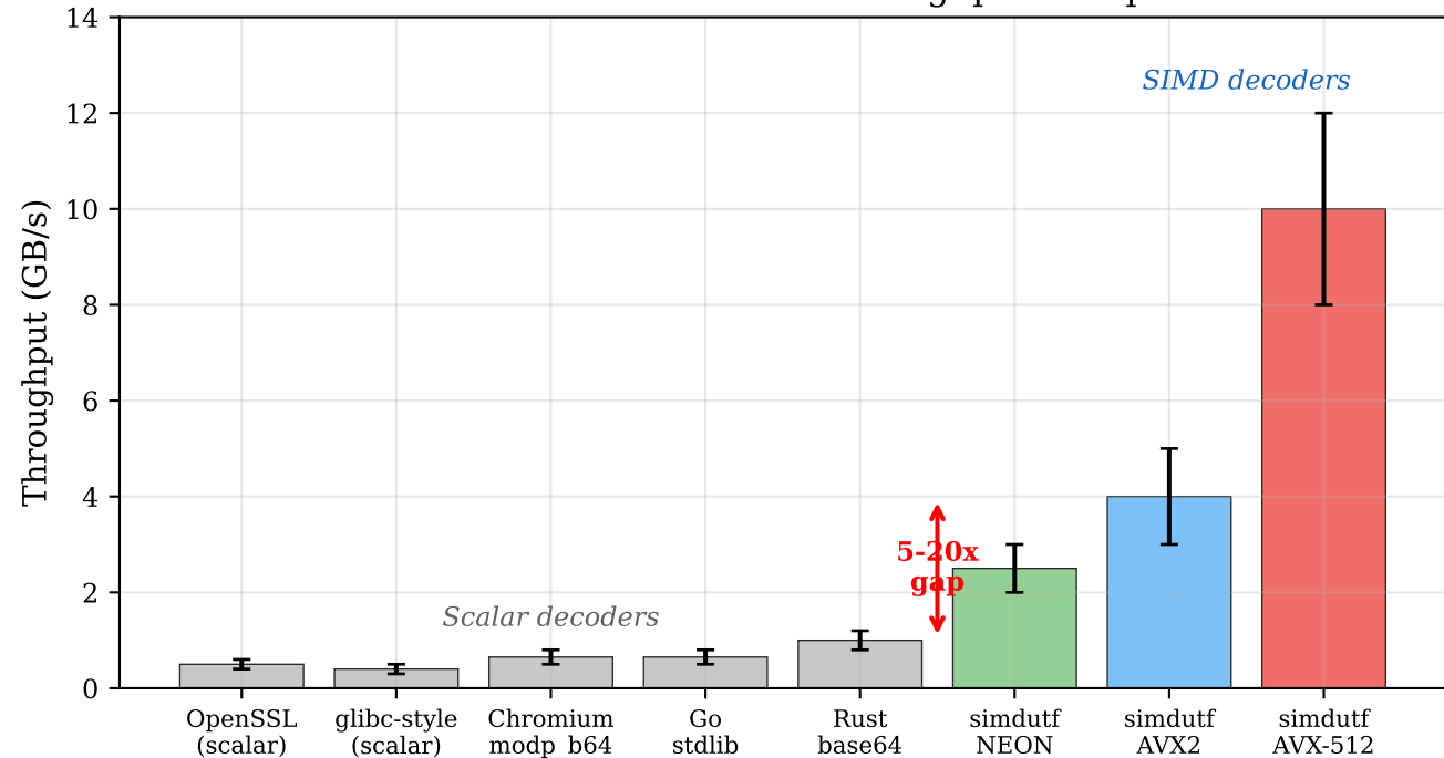
Production Base64 Decoder Throughput Comparison
