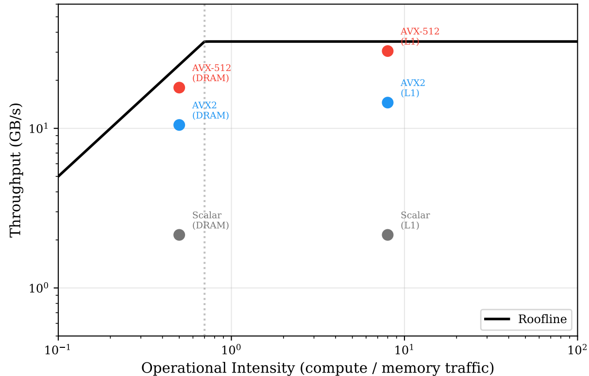
Roofline Model: Base64 Decode Performance
