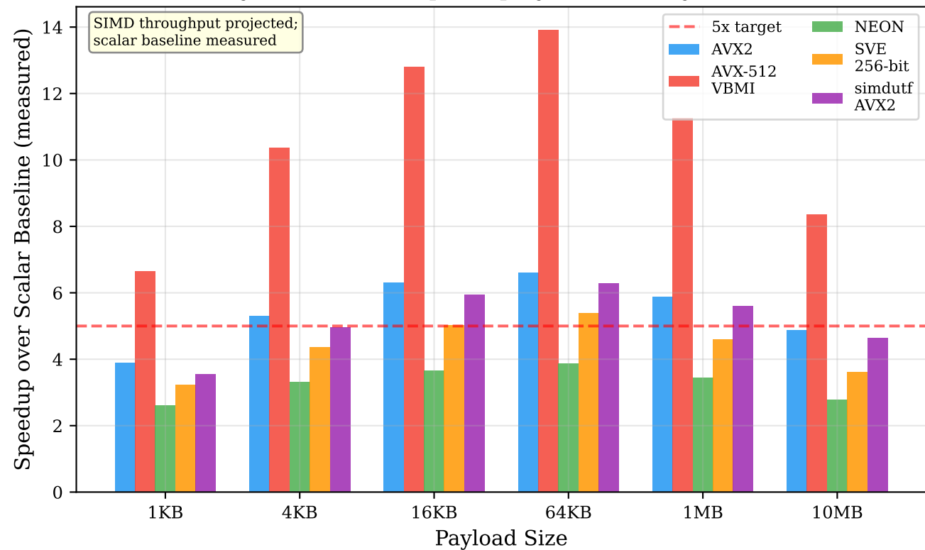
Projected Decode Speedup by ISA and Payload Size
