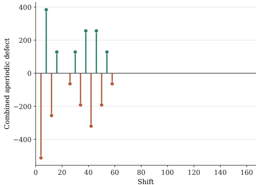
b Published Mod-64 Seed Defects
