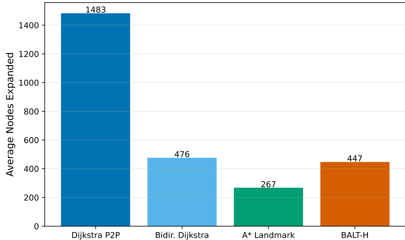
Search Efficiency: Nodes Expanded ( n \geq 1000 )
