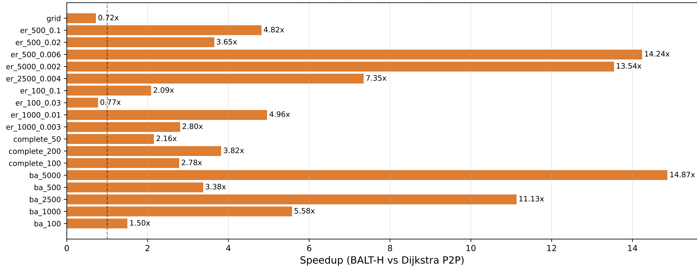
Speedup by Graph Configuration
