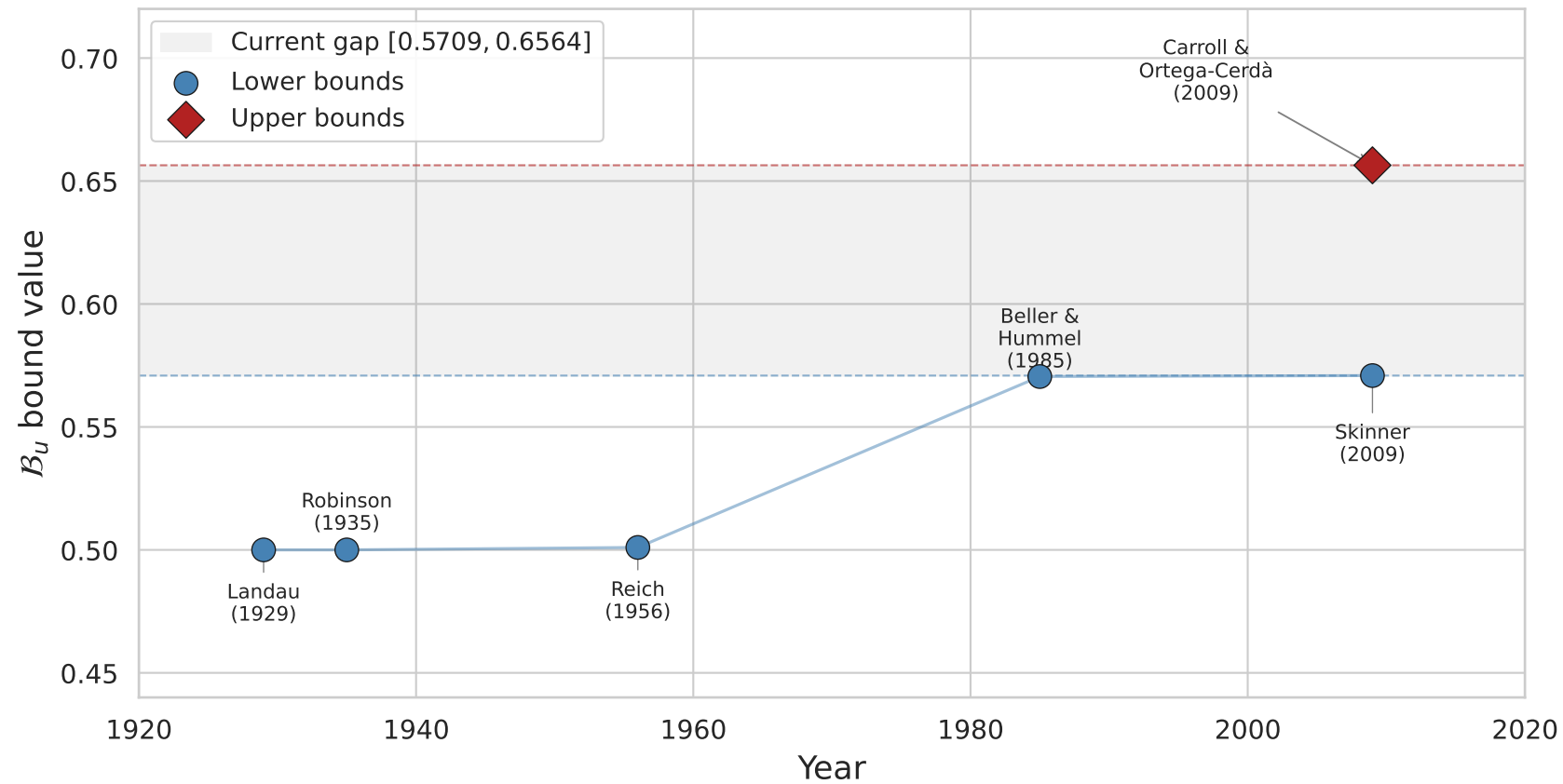
Timeline of bounds on the univalent Bloch constant B_u
