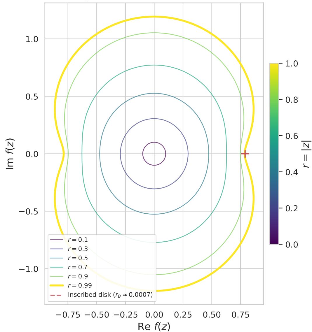
Image domain of f(z) = z - 0.21z^3
