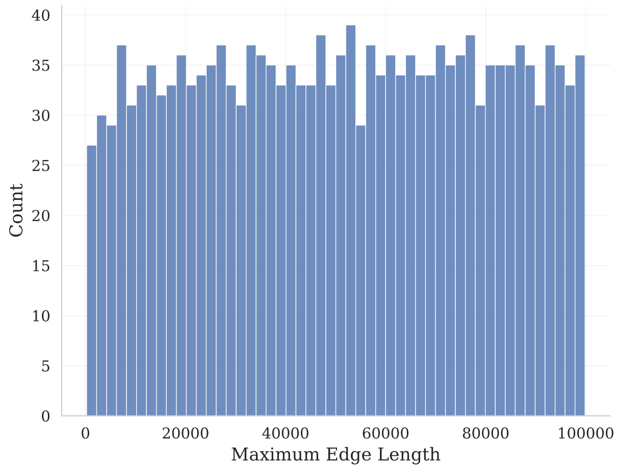
Distribution of Euler Brick Sizes
