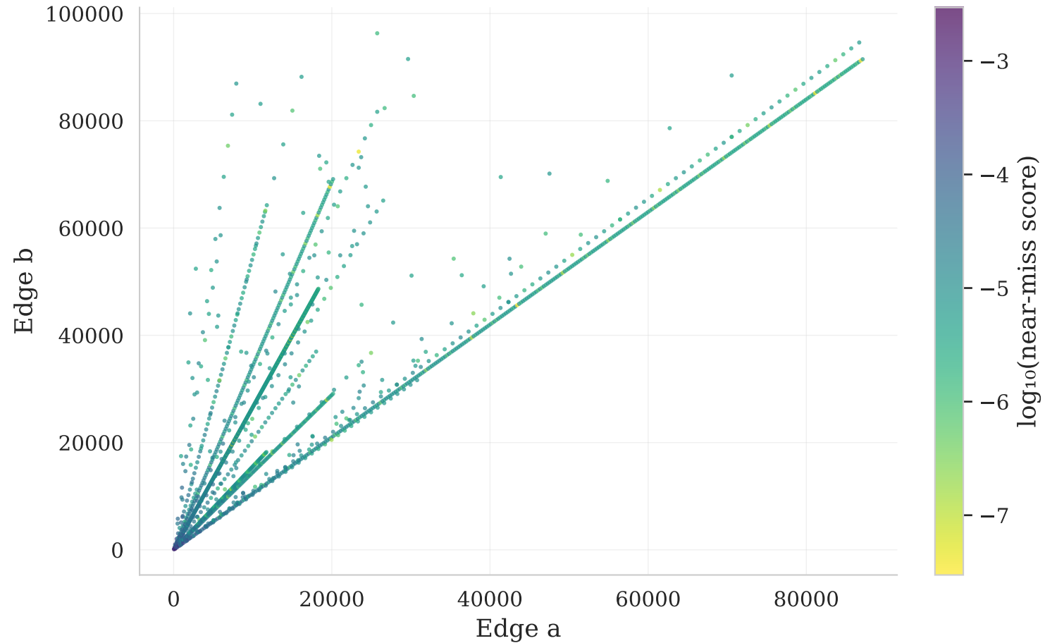
Euler Bricks: a vs b
