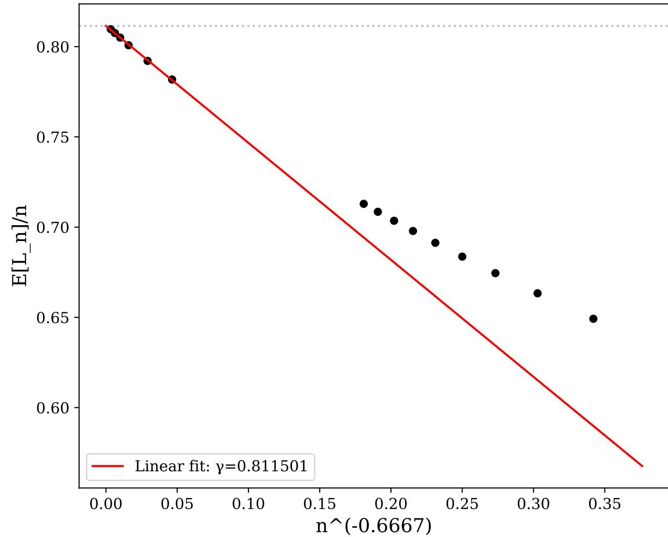
Scaling collapse (Intermediate (beta=2/3))
