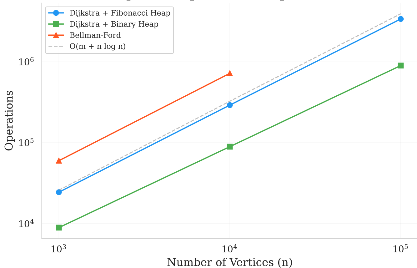
Sparse Graphs — Total Operations
