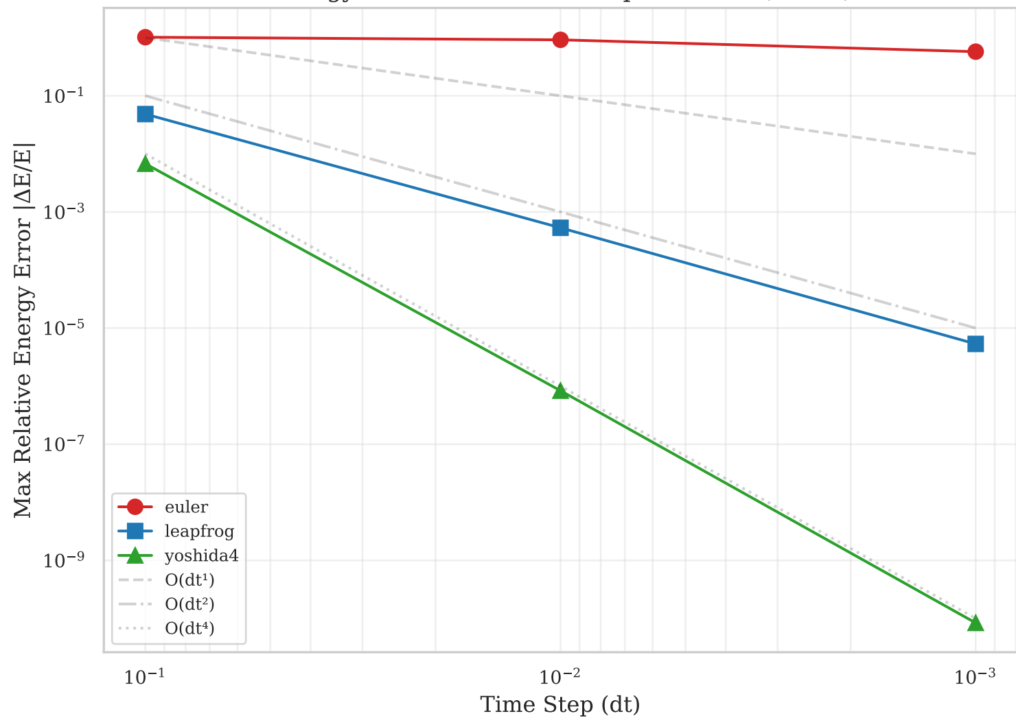
Energy Conservation: 100 Kepler Orbits ( e=0.5 )
