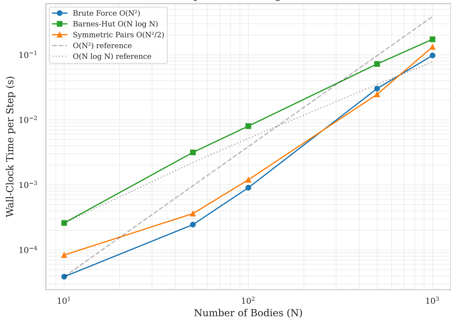
Force Computation Scaling: Runtime vs N
