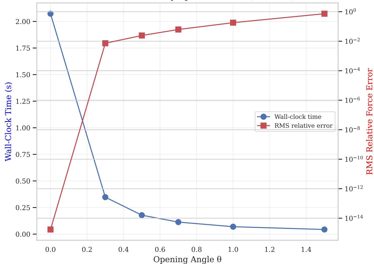
Barnes-Hut Accuracy-Speed Tradeoff (N=1000)
