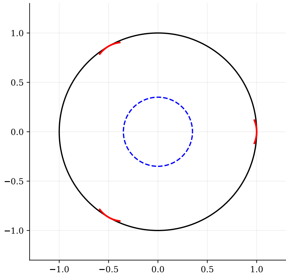
Carroll-Ortega-Cerdà Harmonic Arc Domain B_U \leq 0.6564
