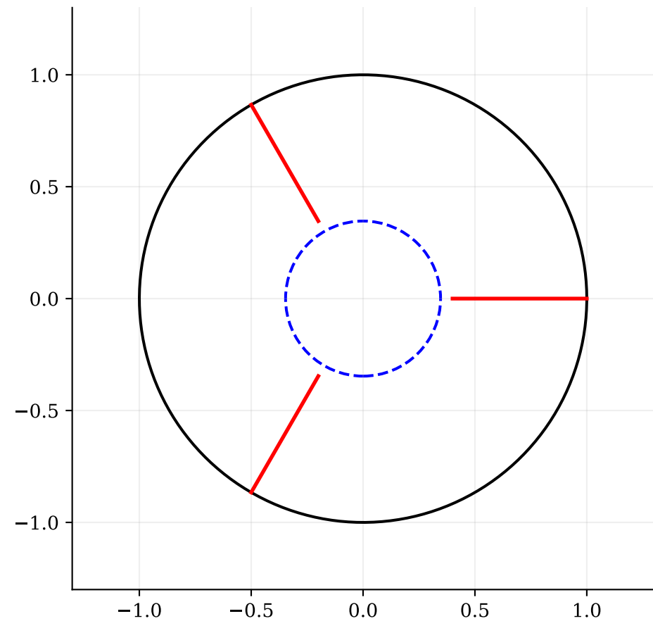
Goodman 3-Slit Domain B_U \leq 0.6565
