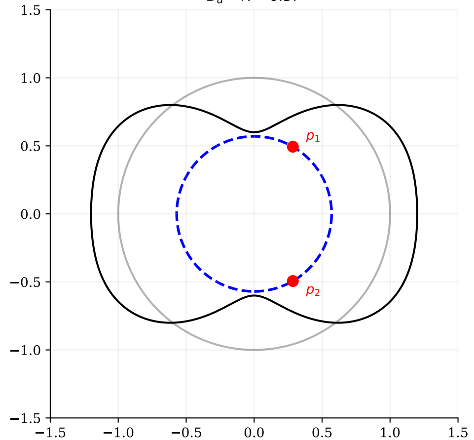
Conjectured Extremal (Jenkins 2-contact-point) B_U = R \approx 0.57
