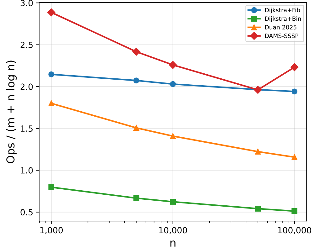
Worst-Case Graphs
