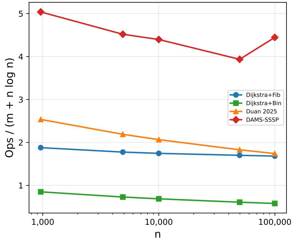
Grid Graphs
