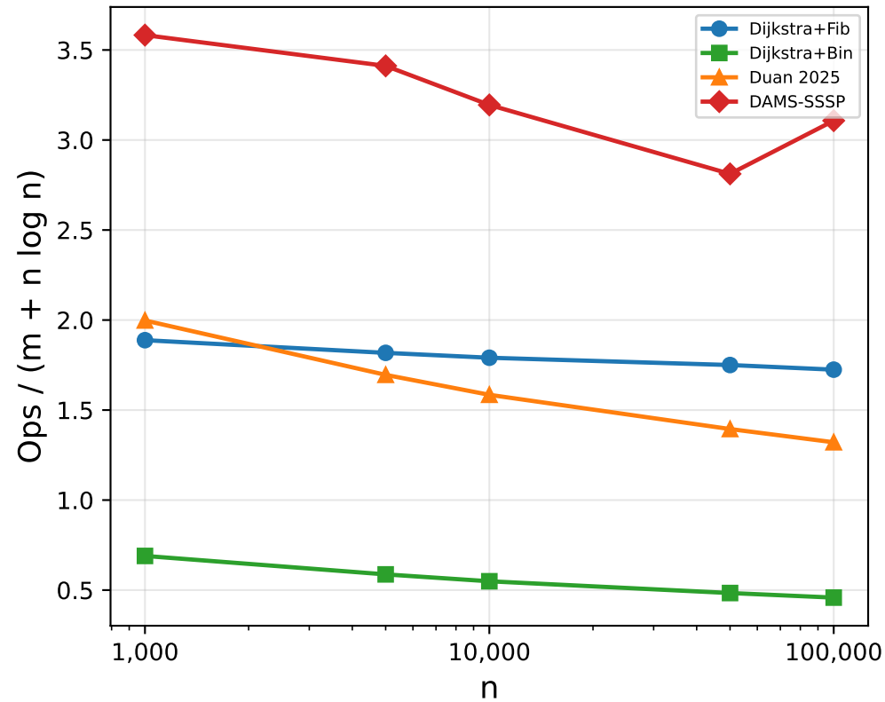
Sparse Graphs
