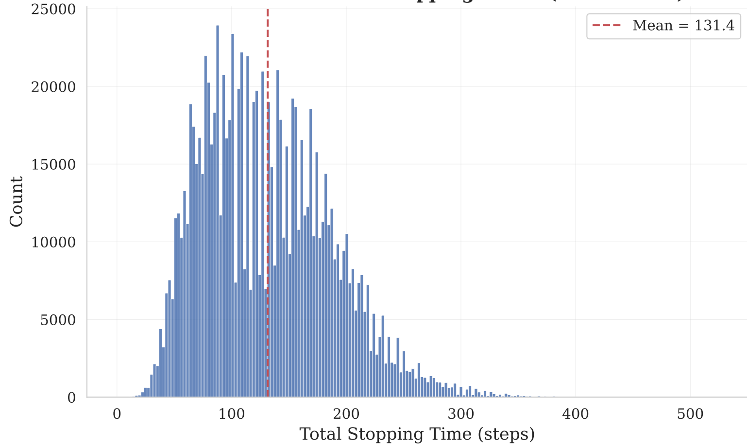
Distribution of Collatz Stopping Times ( n = 1 to 10^6 )
