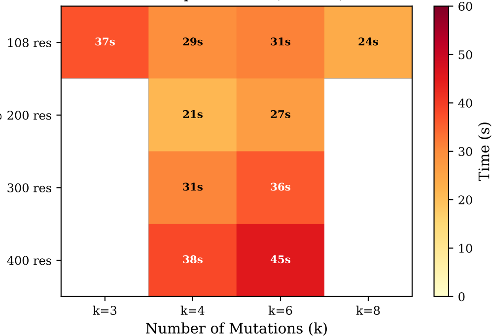
Total Pipeline Time (seconds)
