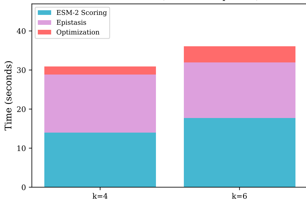
Time Breakdown (300-residue protein)
