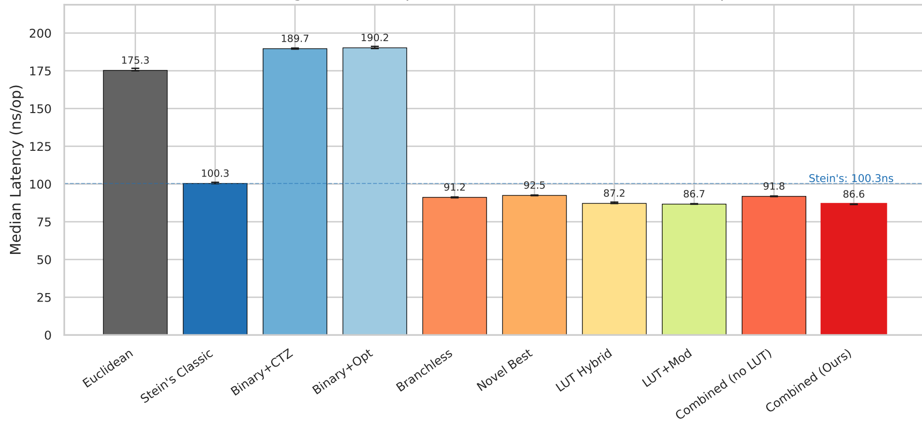
GCD Algorithm Comparison — 64-bit Uniform Random Inputs
