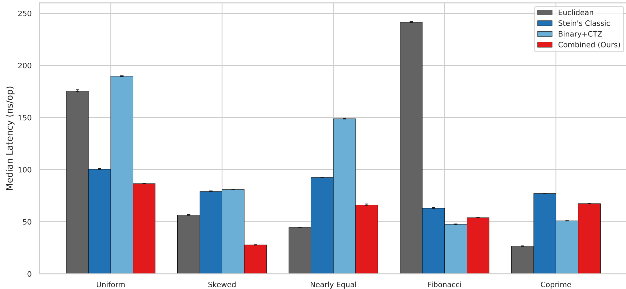
GCD Algorithm Performance Across Input Distributions (64-bit)
