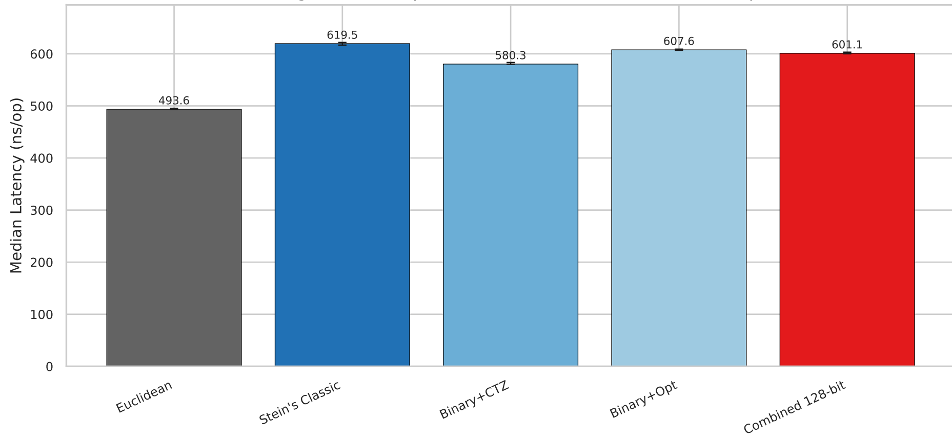
GCD Algorithm Comparison — 128-bit Uniform Random Inputs
