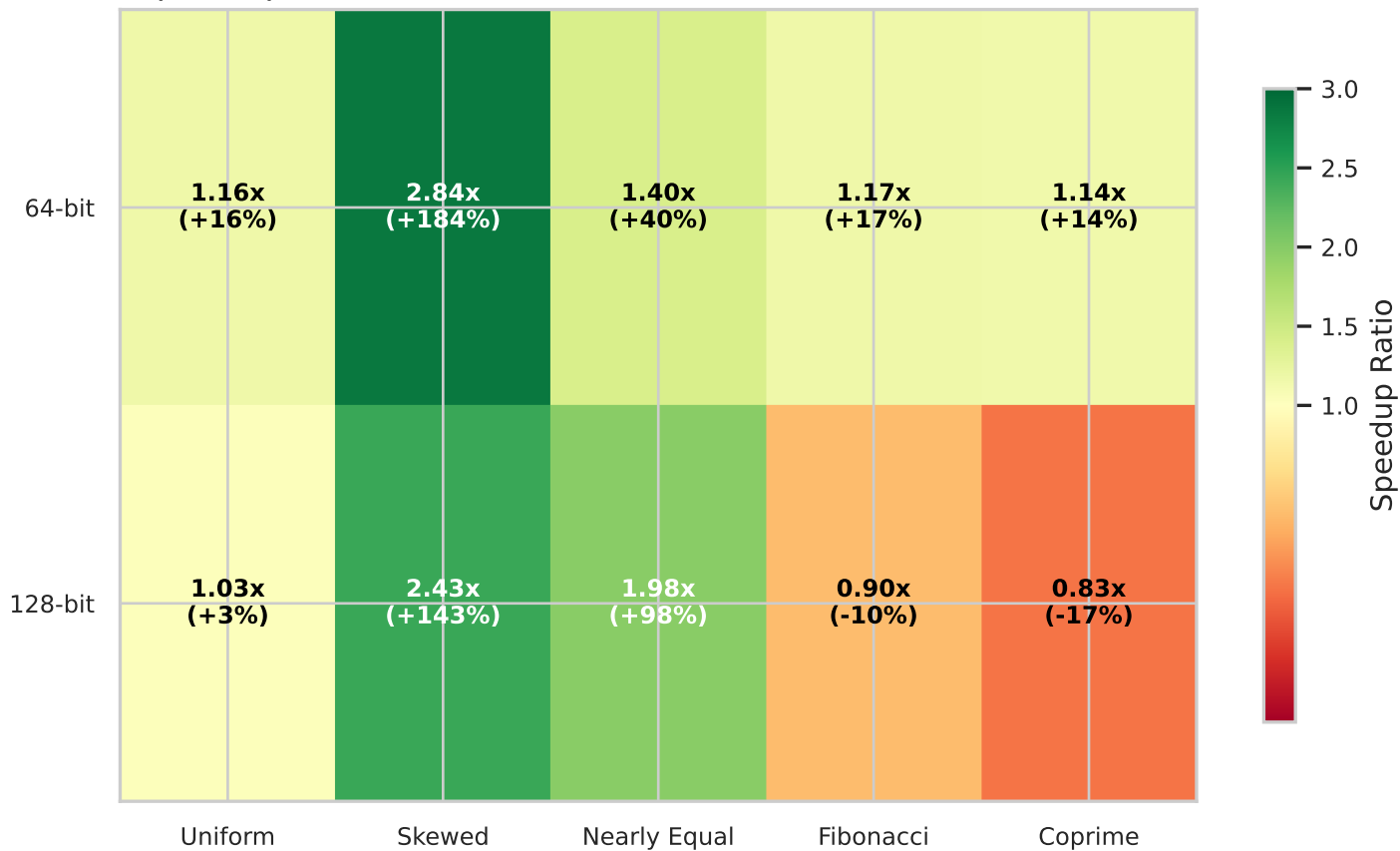
Speedup: Combined / Stein's Classic (>1.0 = novel is faster)
