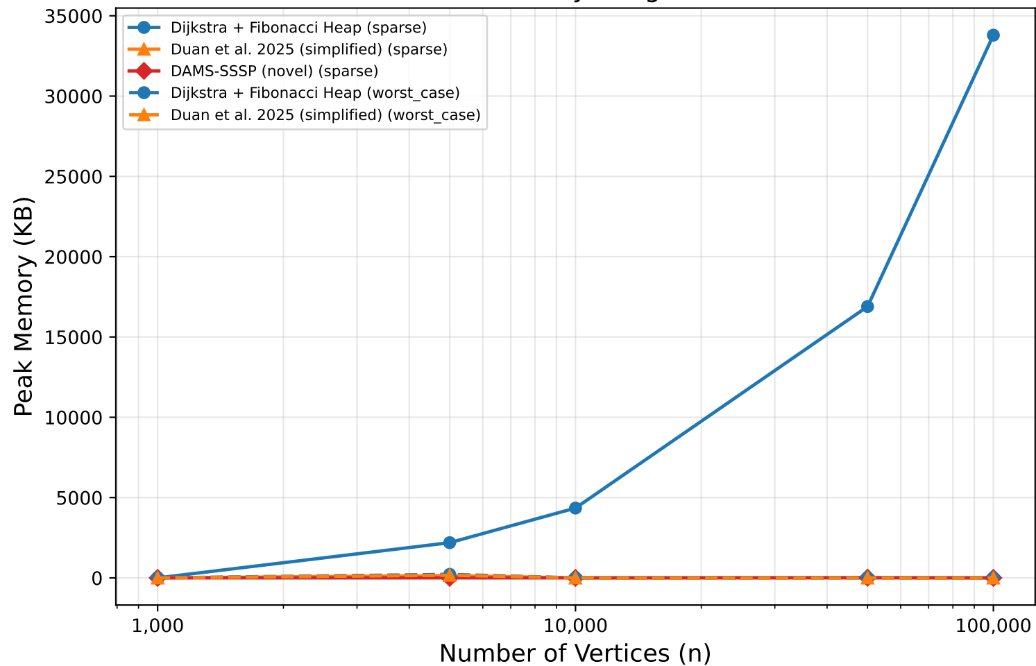
Peak Memory Usage vs n
