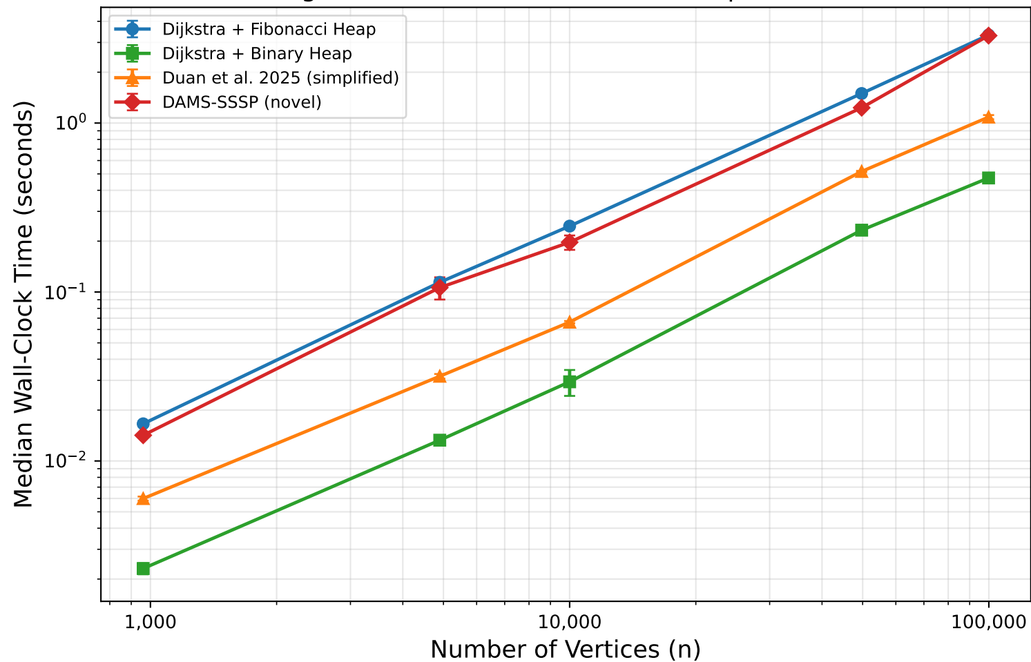
Scaling: Wall-Clock Time vs n (Grid Graphs ( m \approx 4n ))
