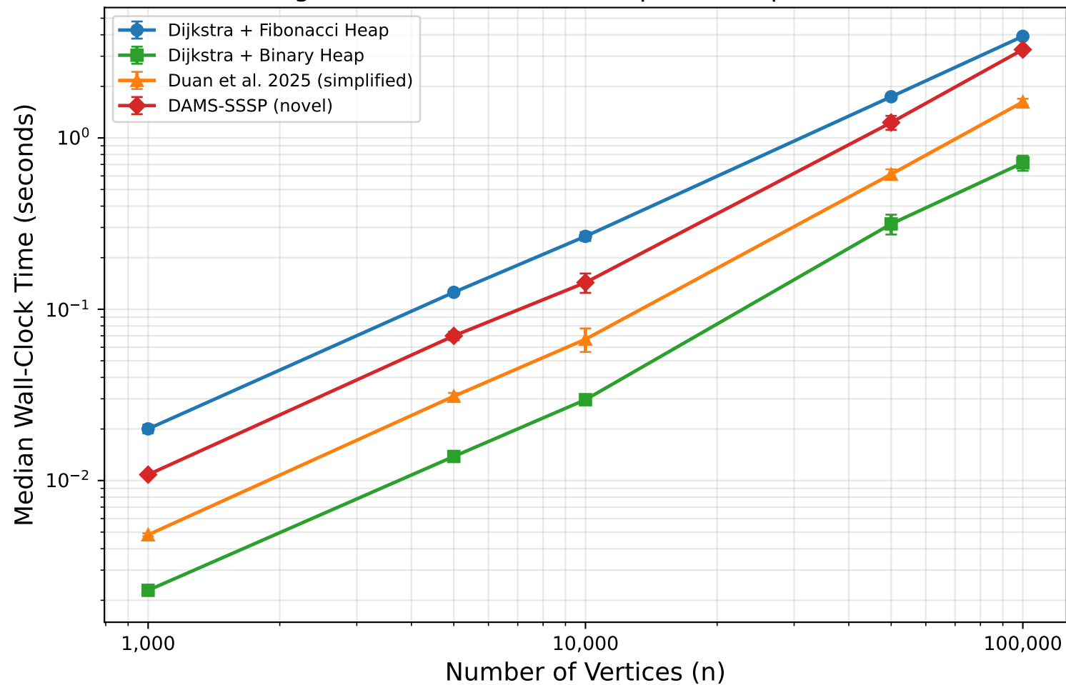
Scaling: Wall-Clock Time vs n (Sparse Graphs ( m = 3n ))
