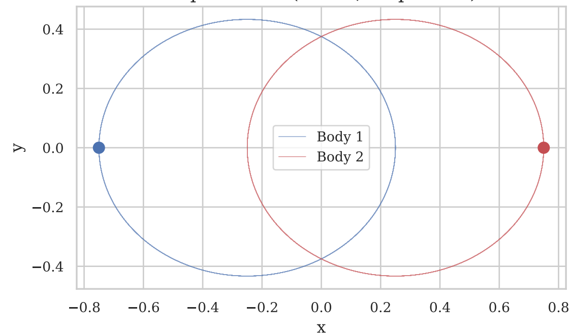
Kepler Orbit (e=0.5, 10 periods)
