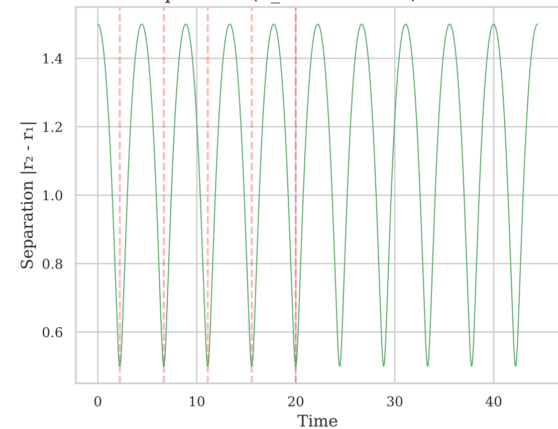
Orbital Separation (T_meas=4.4429, err=0.00e+00)
