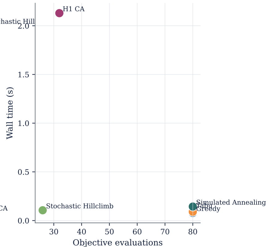
Evaluations vs. wall time
