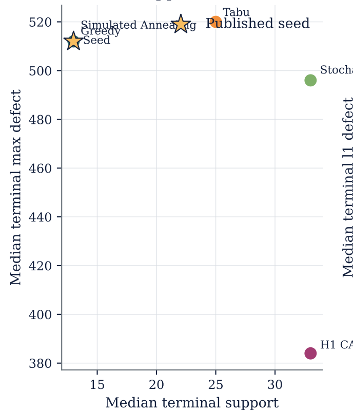
Terminal support vs. max defect
