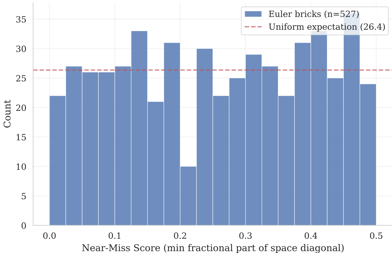
Distribution of Space Diagonal Near-Miss Scores for Euler Bricks
