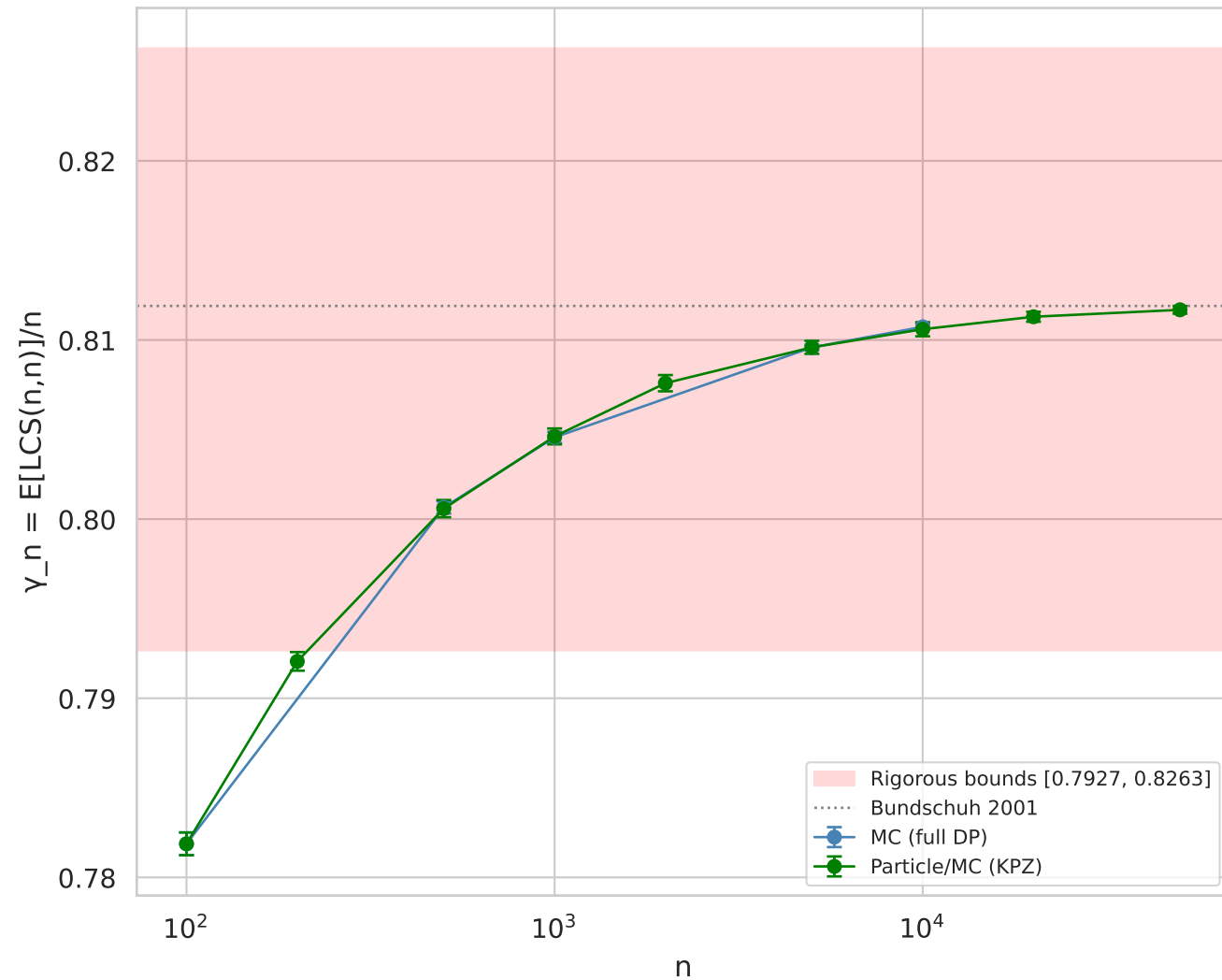
Empirical \gamma_2 Estimates vs. String Length
