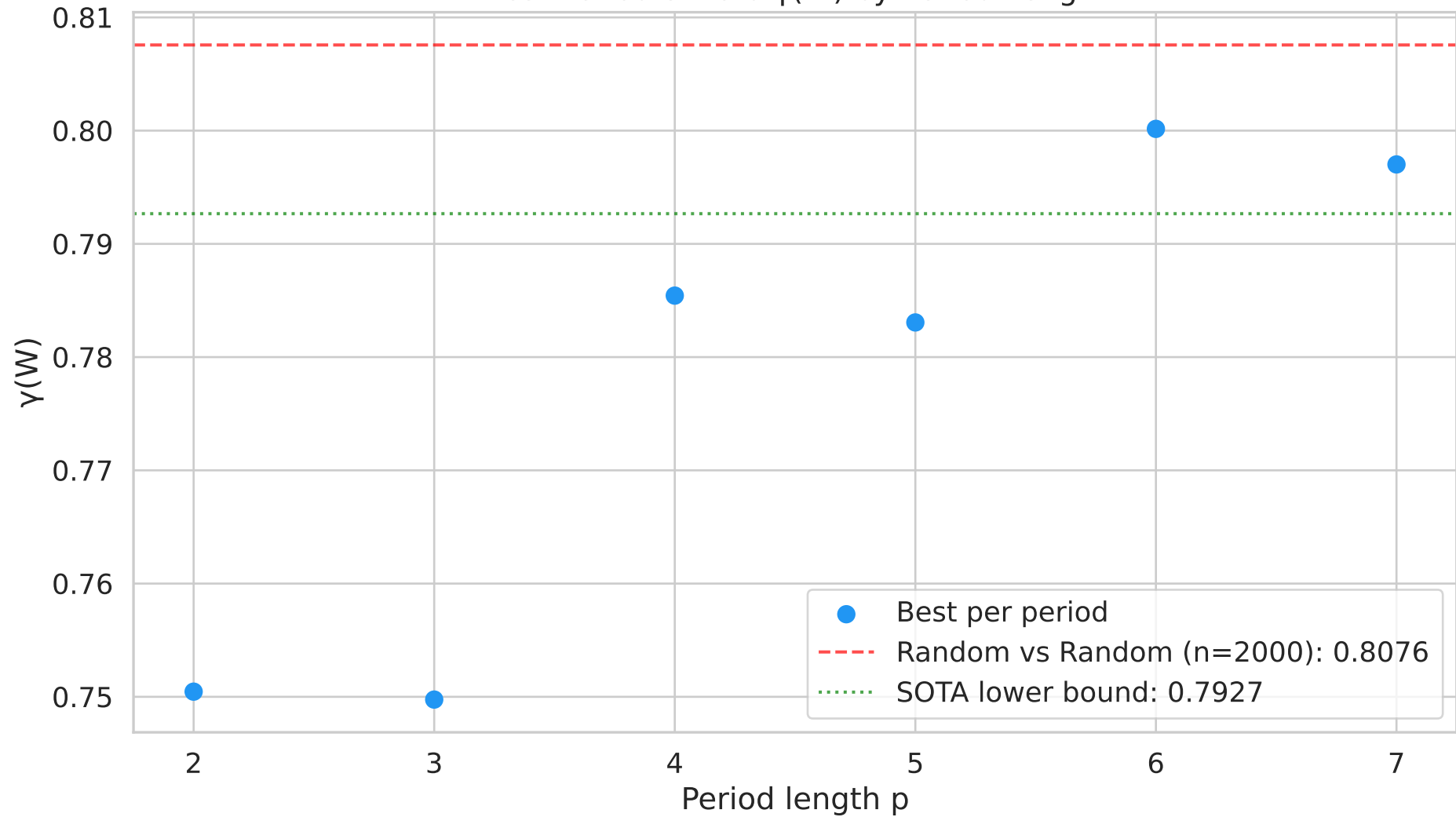
Best Periodic Word \gamma(W) by Period Length
