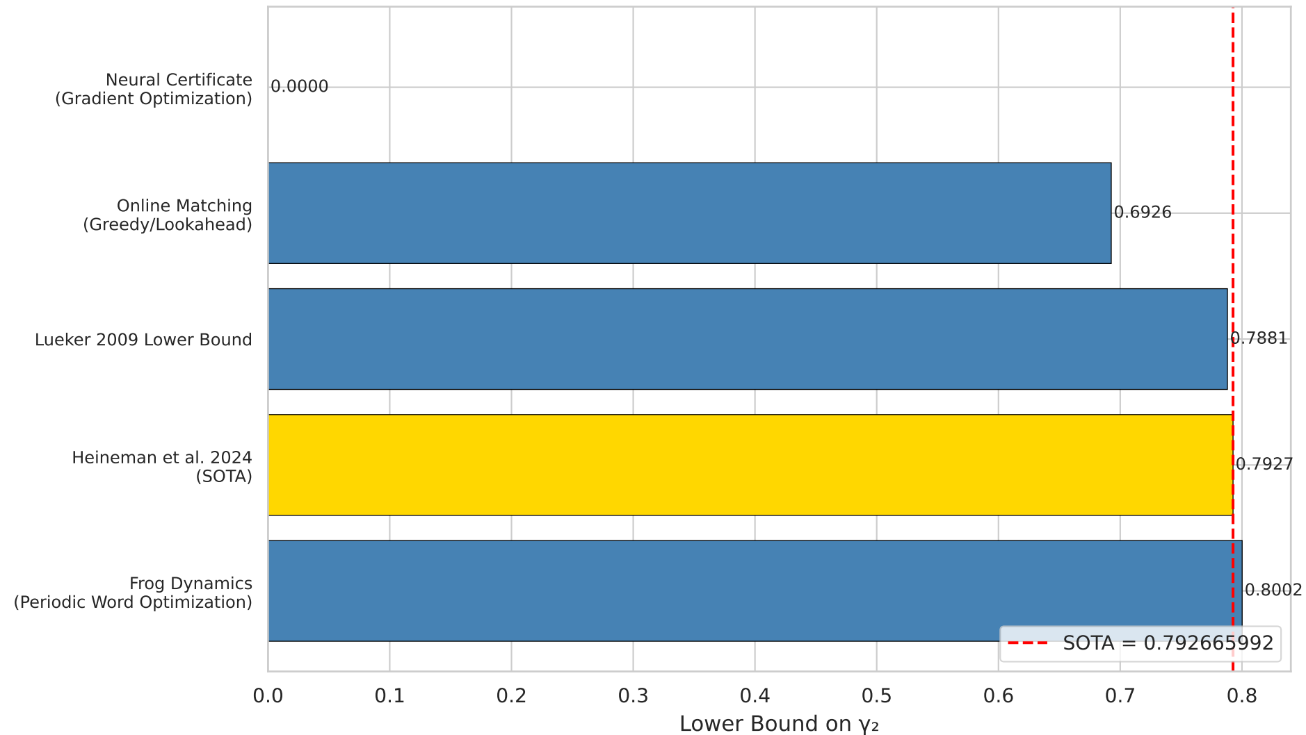
Comparison of Lower Bound Approaches for \gamma_2
