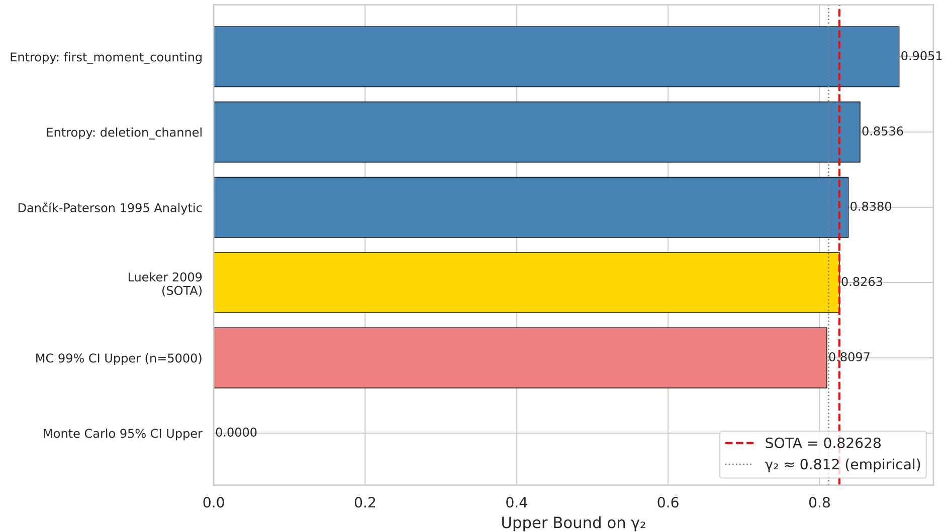
Comparison of Upper Bound Approaches for \gamma_2
