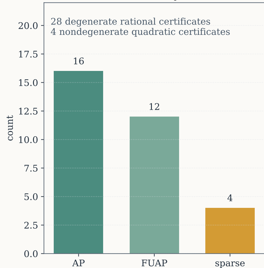
Exact-certified cases by selector family
