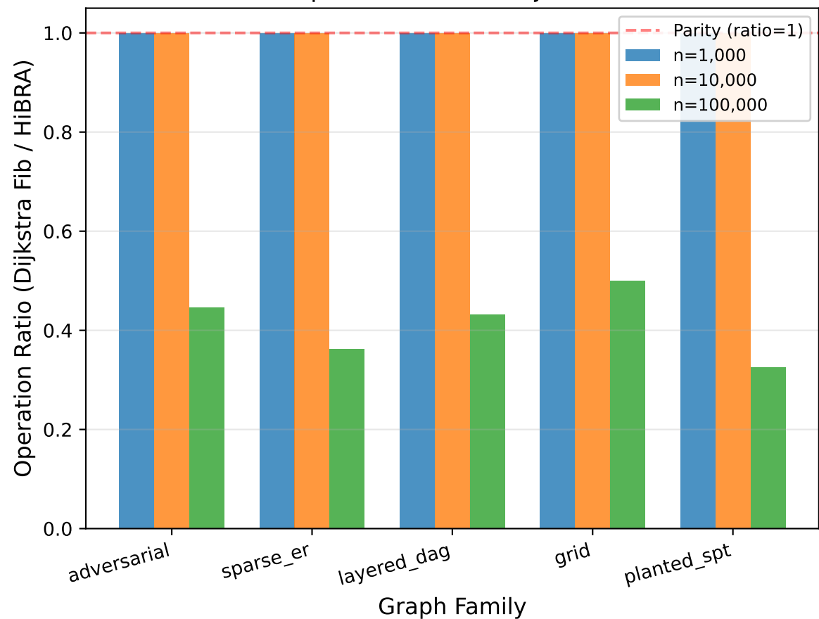
Relative Operation Count: Dijkstra vs HiBRA
