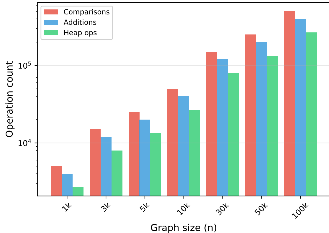
Operation Breakdown: Dijkstra (binary heap)
