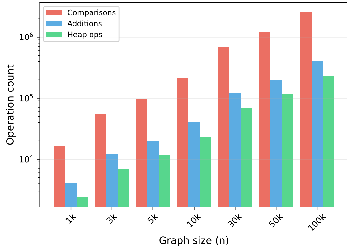
Operation Breakdown: HiBRA (k-ary Fib)
