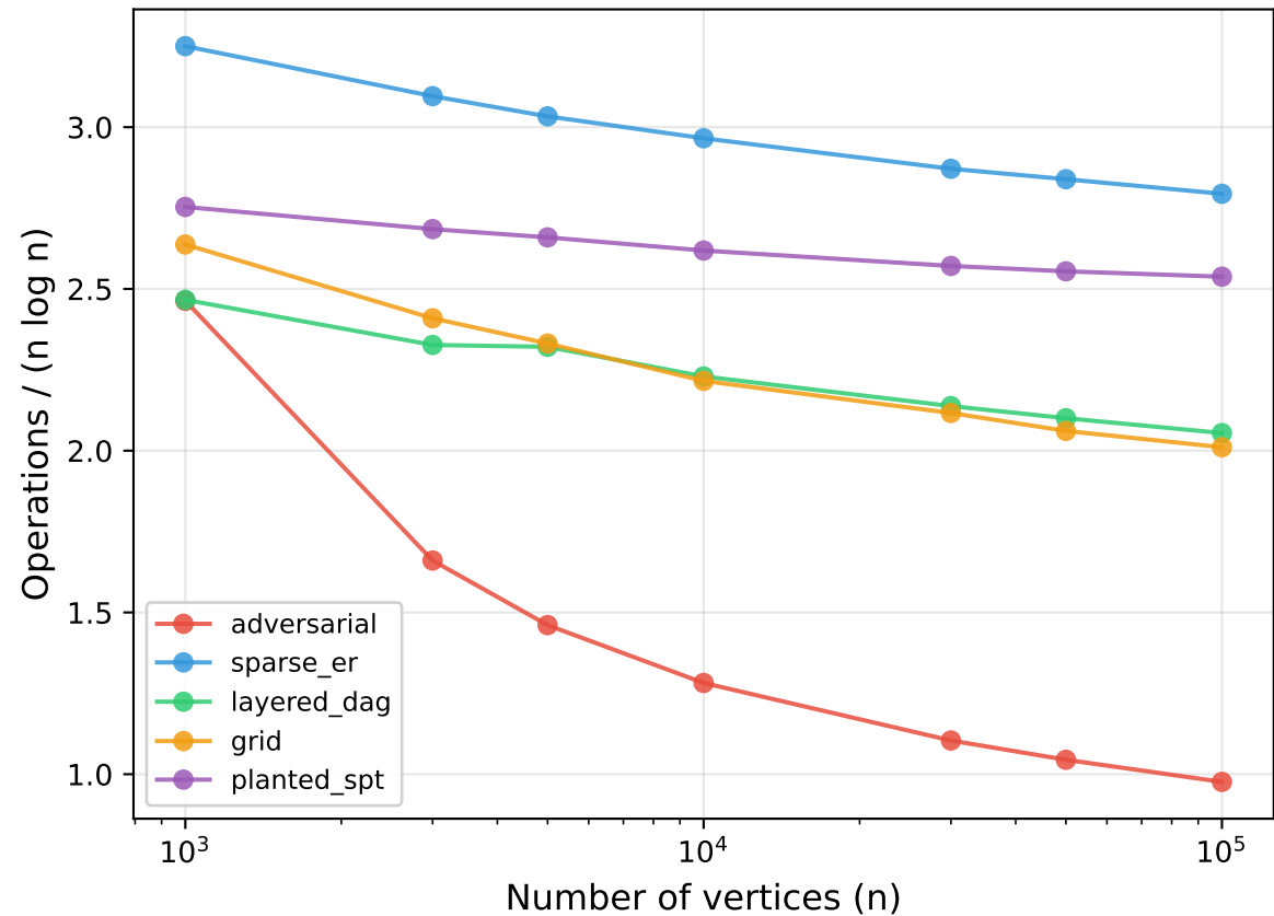
HiBRA: Normalized Operation Count Across Graph Families
