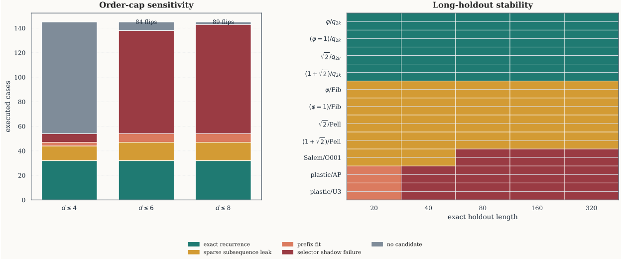
Figure 7: Claim-sensitive ablations requested by the verification audit. Left: raising the search ceiling from d \leq 4 to d \leq 6 and d \leq 8 adds no new exact-certified case, but it converts many former no_candidate rows into higher-order short-window fits and modular-shadow failures. This is why the paper does not infer new mathematics from a larger order cap alone. Right: longer holdouts. The four certified quadratic-convergent identities remain exact through lengths 40, 80, 160, and 320; the unresolved Fibonacci/Pell quadratic cases also retain exact holdouts empirically; the three plastic prefix fits fail by 40, and saalem_quartic / ost_suffix_001 fails by 80.
