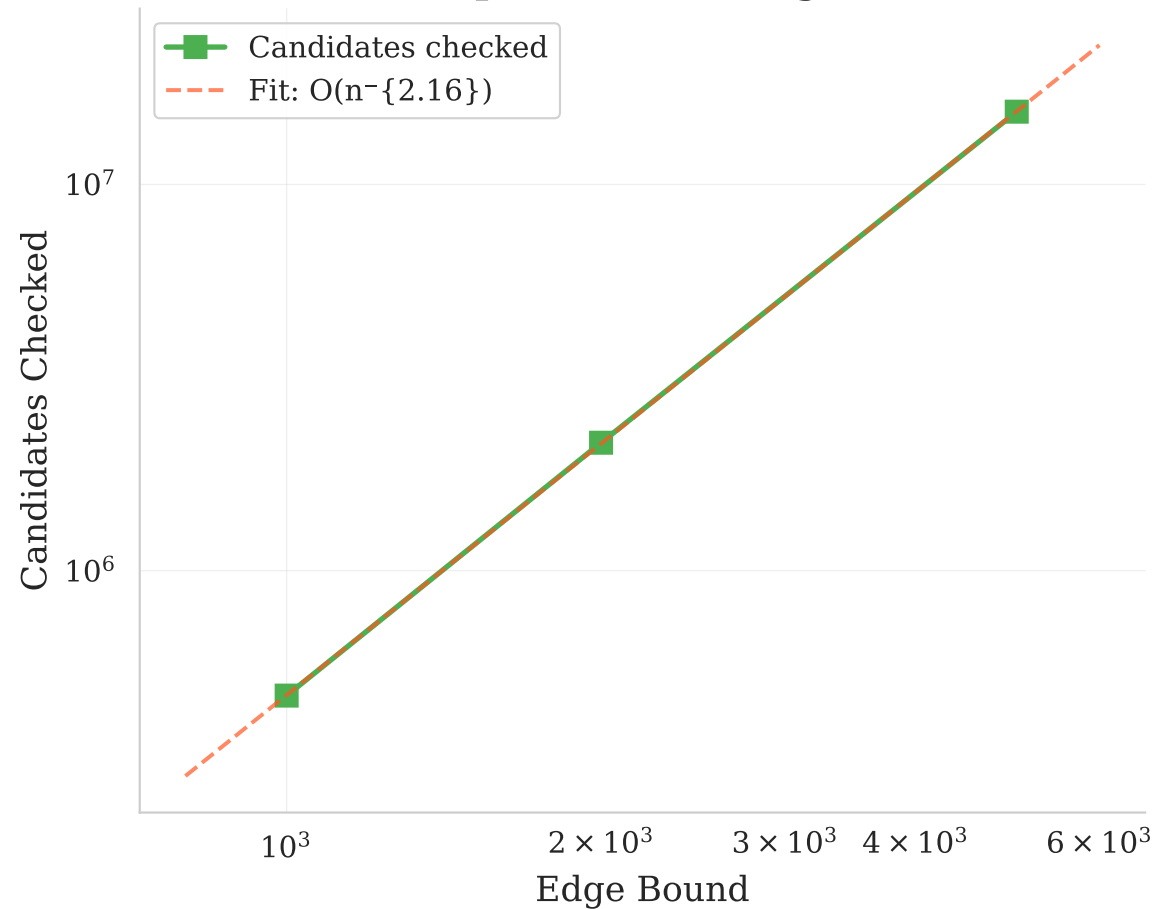
Search Space Size vs Edge Bound
