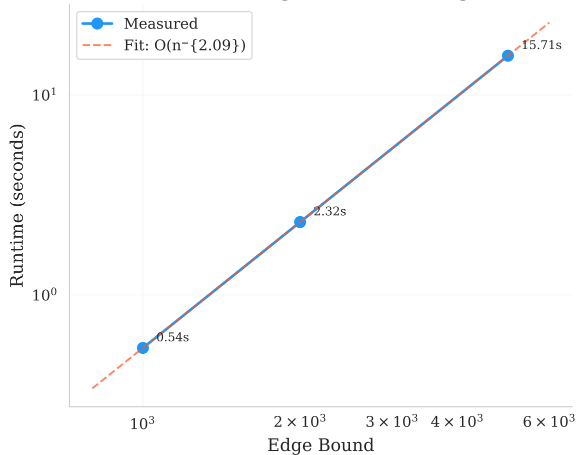
Brute Force Scaling: Runtime vs Edge Bound
