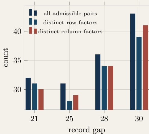
A. Full witness hypergraphs stay sparse
