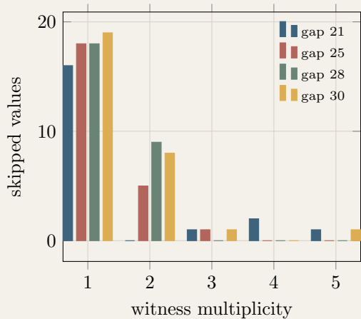
B. Singleton-dominated multiplicity persists
